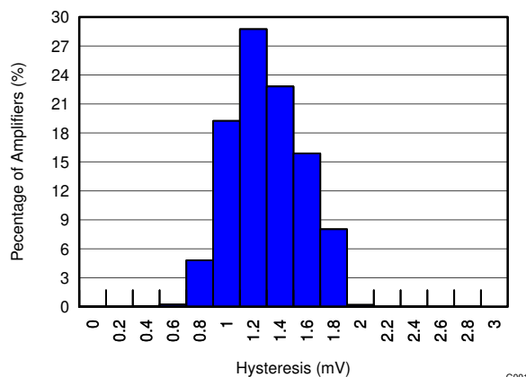
Figure 6-2. Hysteresis Distribution
