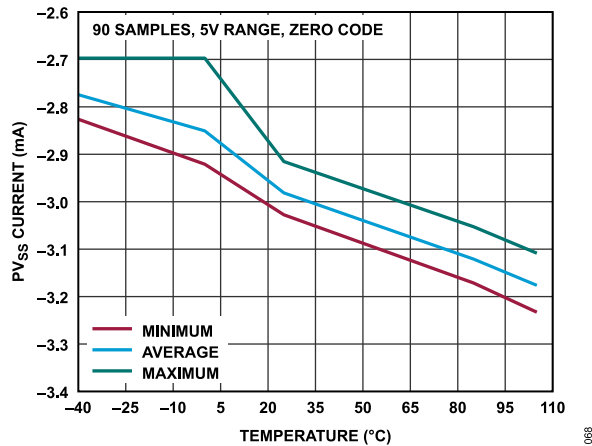
Figure 75. PV_{SS} Current vs. Temperature
