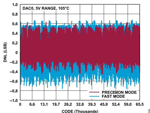
Figure 13. AD3541R-16 DNL vs. Code, 0 V to 5 V Range, 105^{\circ}\text{C} , Fast Mode and Precision Mode
