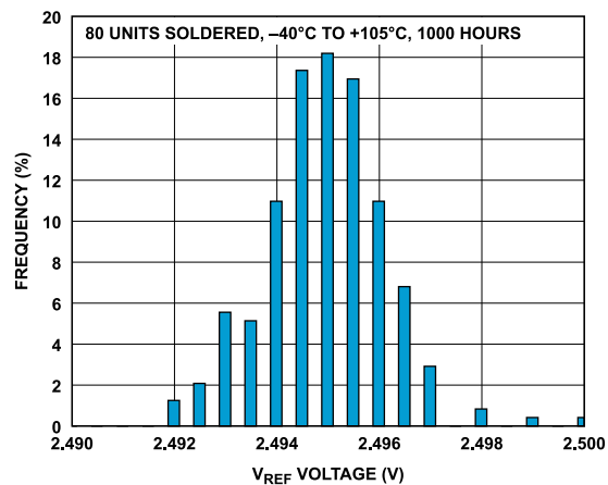
Figure 66. Reference Voltage Spread
