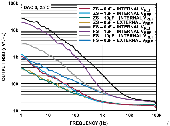
Figure 30. Output Noise Spectral Density (NSD) vs. Frequency
