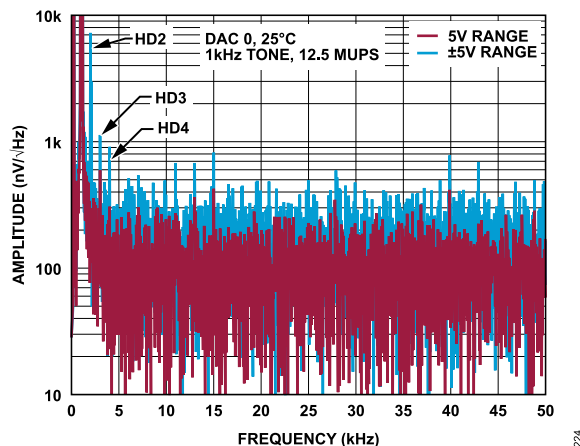
Figure 36. AD3541R-16 Spectral Noise Density with 1 kHz Sine Wave Playback (HD2 Is Second Harmonic Distortion, HD3 Is Third Harmonic Distortion, HD4 Is Fourth Harmonic Distortion)
