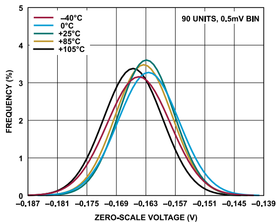
Figure 42. Zero-Scale Voltage Distribution, 0 V to 10 V Range
