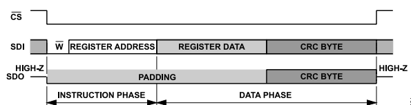
Figure 86. Basic SPI Write Frame with CRC
