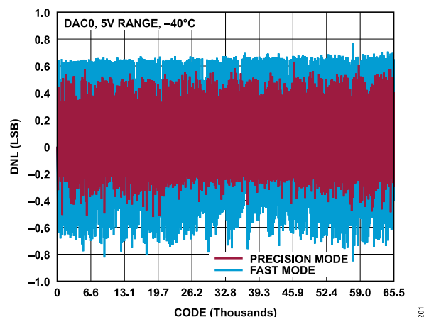
Figure 10. AD3541R-16 DNL vs. Code, 0 V to 5 V Range, -40^{\circ}\text{C} , Fast Mode and Precision Mode
