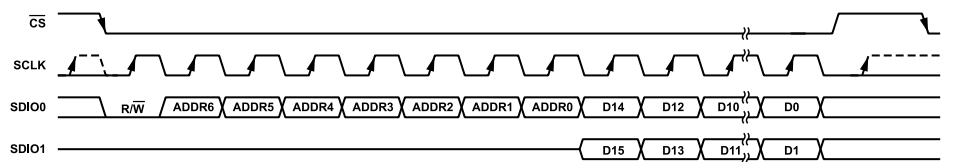
Figure 91. Dual SPI Mode
