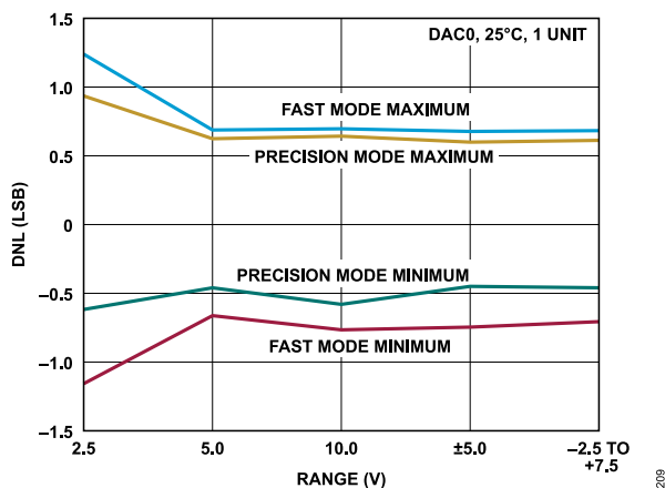
Figure 20. AD3541R-16 DNL vs. Range, Fast Mode and Precision Mode
