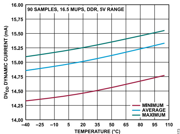
Figure 73. AD3541R-12 DV_{DD} Dynamic Current vs. Temperature
