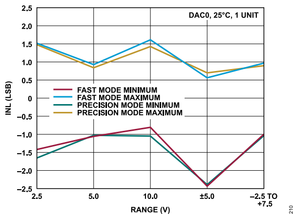
Figure 21. AD3541R-16 INL vs. Range, Fast Mode and Precision Mode
