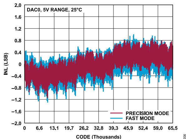
Figure 16. AD3541R-16 INL vs. Code, 0 V to 5 V Range, 25°C, Fast Mode and Precision Mode
