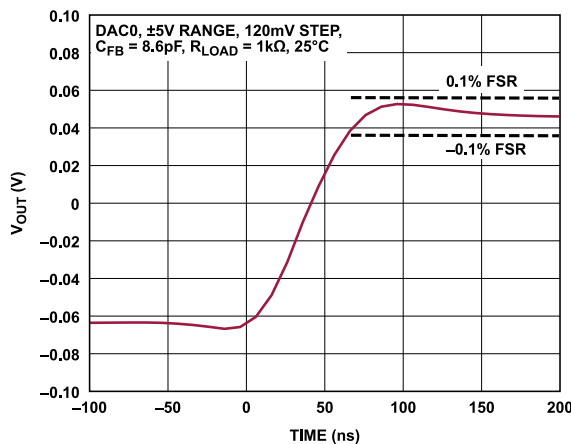
Figure 57. Small Signal Settling Time, -5 V to +5 V Range
