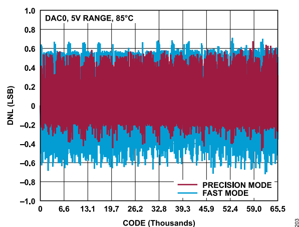
Figure 12. AD3541R-16 DNL vs. Code, 0 V to 5 V Range, 85^{\circ}\text{C} , Fast Mode and Precision Mode
