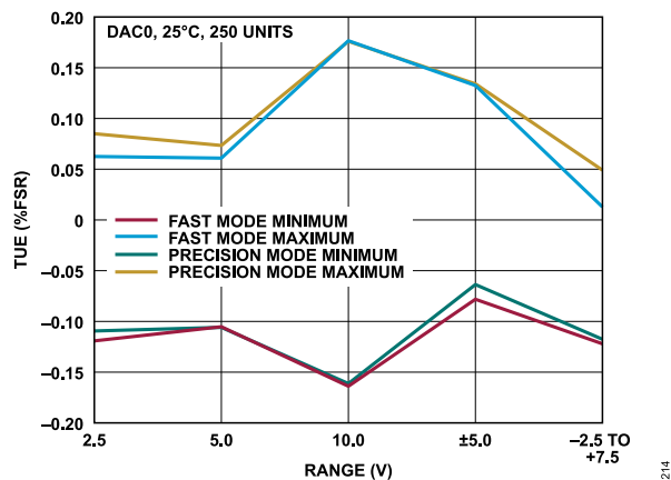
Figure 25. TUE vs. Range
