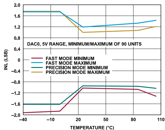
Figure 23. AD3541R-16 INL vs. Temperature
