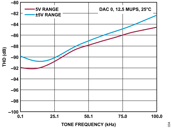
Figure 33. AD3541R-12 THD vs. Tone Frequency
