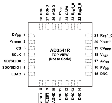
Figure 9. Pin Configuration
