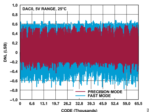
Figure 11. AD3541R-16 DNL vs. Code, 0 V to 5 V Range, 25^{\circ}\text{C} , Fast Mode and Precision Mode
