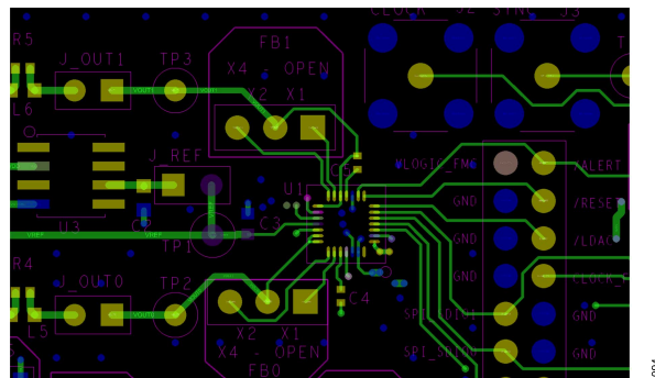
Figure 97. EVAL-AD3542R Component Arrangement and Layout
