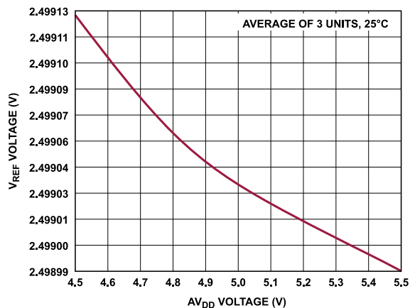
Figure 64. V_{REF} Voltage vs. AV_{DD} Voltage
