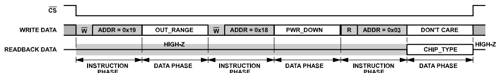
Figure 82. Single Instruction Mode Register Access Example with Address Descending
