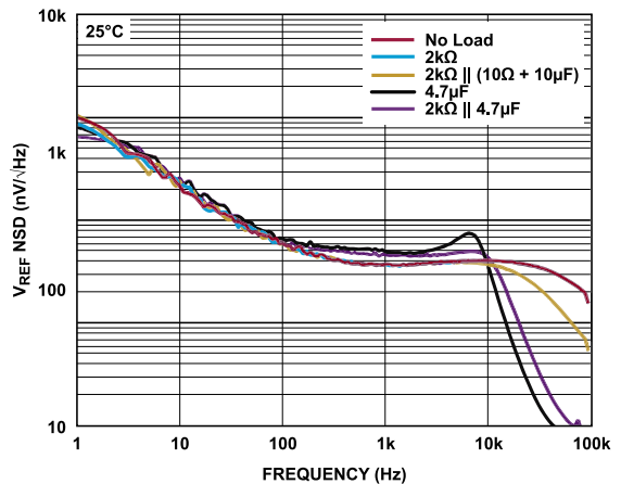
Figure 63. Reference Voltage ( V_{REF} ) NSD vs. Frequency, Load Impedance
