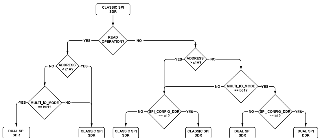
Figure 95. Register Access Modes
