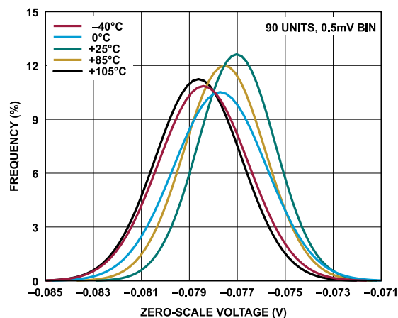
Figure 41. Zero-Scale Voltage Distribution, 0 V to 5 V Range
