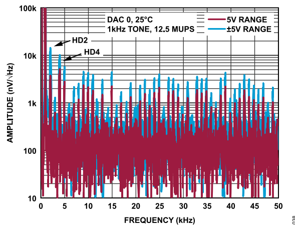
Figure 37. AD3541R-12 Spectral Noise Density with 1 kHz Sine Wave Playback
