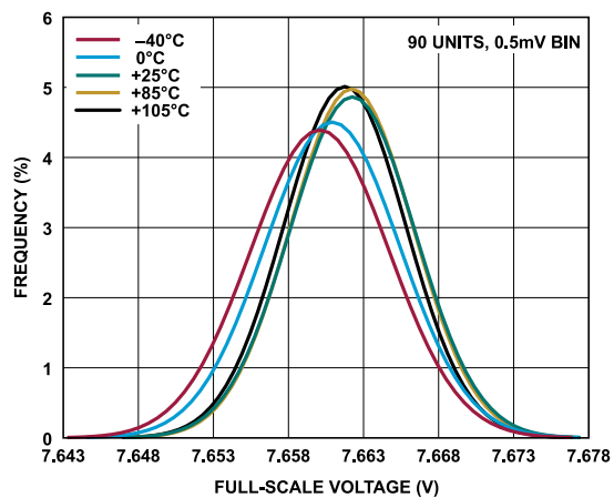
Figure 49. Full-Scale Voltage Distribution, -2.5 V to +7.5 V Range
