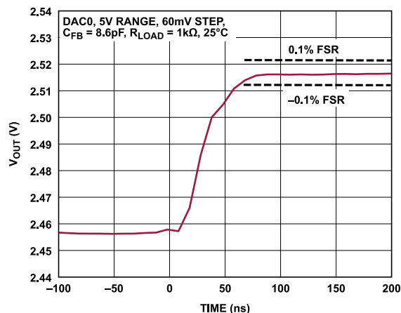
Figure 55. Small Signal Settling Time, 0 V to 5 V Range ( R_{LOAD} Is Load Resistance)
