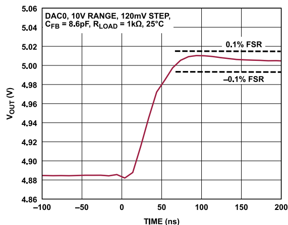
Figure 56. Small Signal Settling Time, 0 V to 10 V Range
