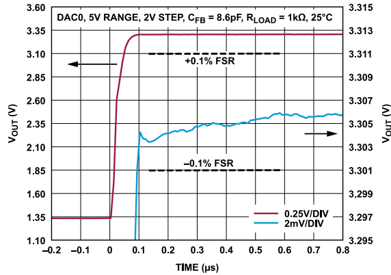
Figure 58. Large Signal Settling Time, 0 V to 5 V Range
