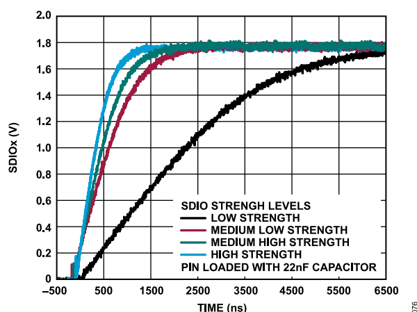
Figure 93. Driving Strength Options
