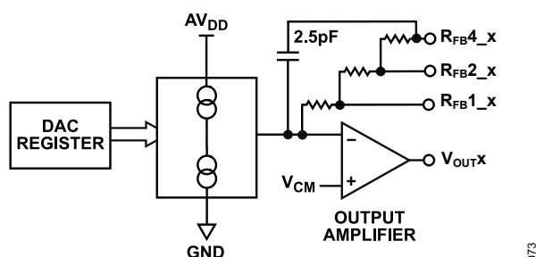
Figure 77. DAC Channel Architecture Block Diagram
