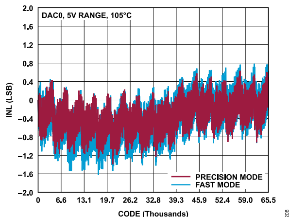
Figure 18. AD3541R-16 INL vs. Code, 0 V to 5 V Range, 105°C, Fast Mode and Precision Mode
