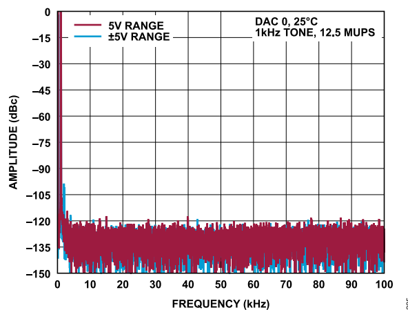
Figure 38. AD3541R-16 Fast Fourier Transform (FFT) with 1 kHz Sine Wave, 12.5 MUPS
