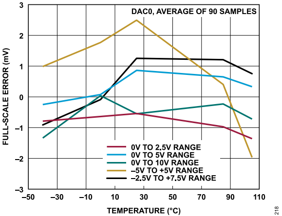
Figure 29. Full-Scale Error vs. Temperature
