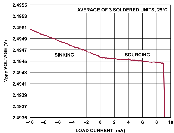
Figure 65. V_{REF} Voltage vs. Load Current
