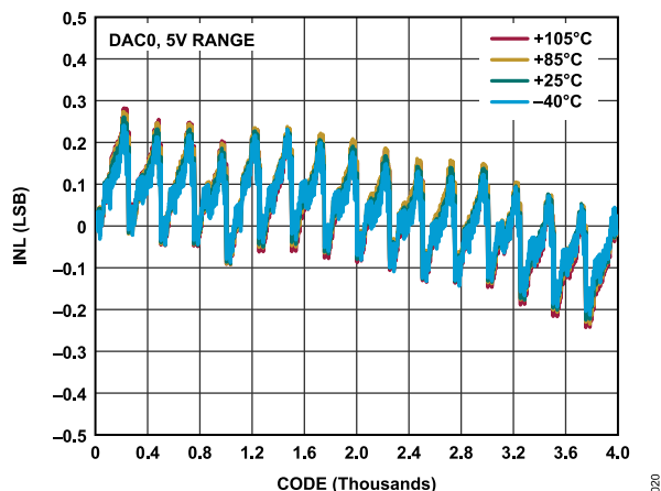
Figure 19. AD3541R-12 INL vs. Code vs. Temperature, 0 V to 5 V Range
