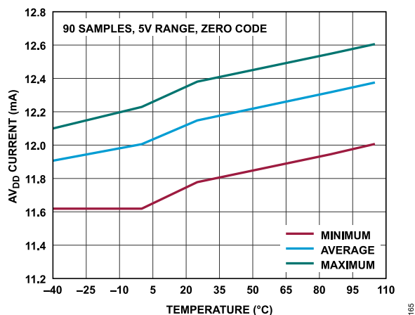
Figure 71. AV_{DD} Current vs. Temperature
