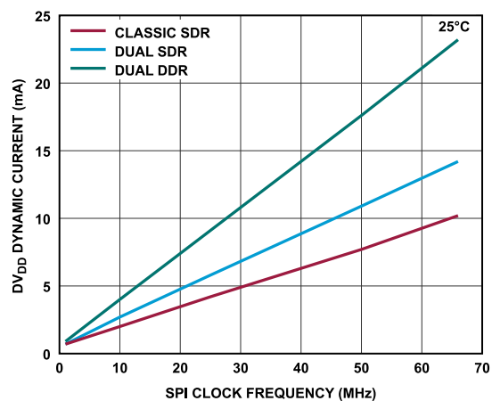
Figure 68. AD3541R-16 DV_{DD} Dynamic Current vs. SPI Clock Frequency, SPI Mode
