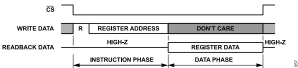
Figure 79. Basic SPI Read Frame
