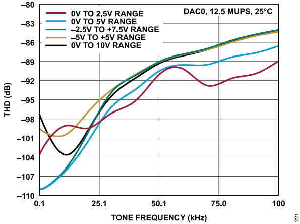
Figure 32. AD3541R-16 THD vs. Tone Frequency
