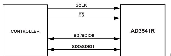
Figure 90. Dual SPI Connection
