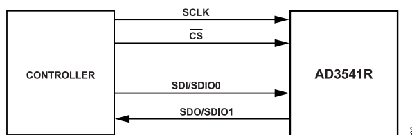
Figure 89. Single SPI (Classic SPI) Connection
