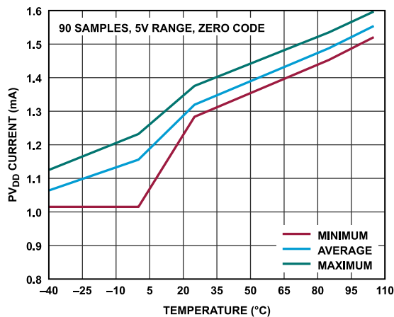
Figure 74. PV_{DD} Current vs. Temperature
