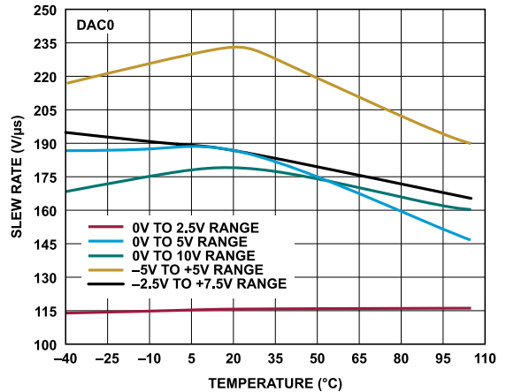
Figure 61. Slew Rate vs. Temperature
