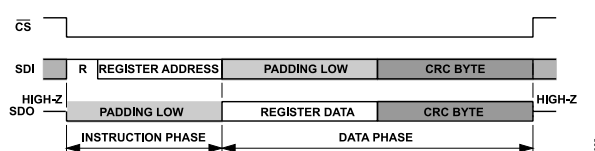
Figure 87. Basic SPI Read Frame with CRC
