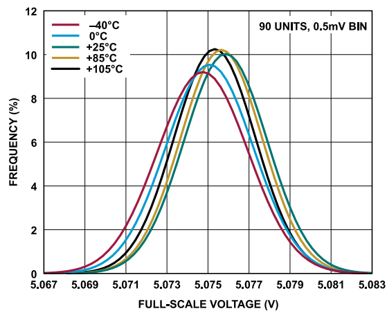
Figure 46. Full-Scale Voltage Distribution, 0 V to 5 V Range
