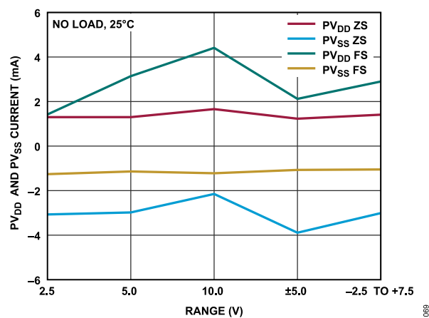
Figure 76. PV DD and PV SS Current vs. Range
