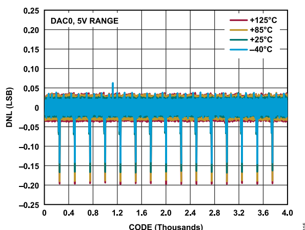
Figure 14. AD3541R-12 DNL vs. Code vs. Temperature, 0 V to 5 V Range
