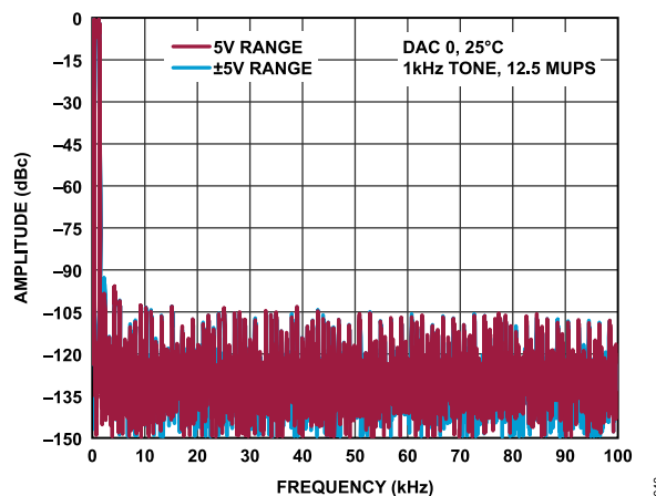
Figure 39. AD3541R-12 Fast Fourier Transform (FFT) with 1 kHz Sine Wave, 12.5 MUPS
