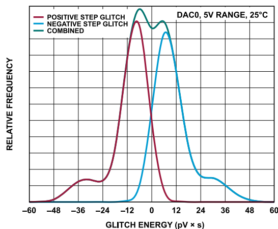
Figure 53. Digital-to-Analog Glitch Energy Histogram
