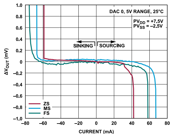
Figure 50. Source and Sink Capability, 5 V Range
