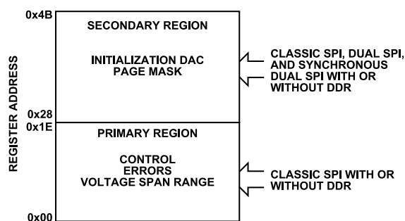
Figure 92. Register Access Modes
