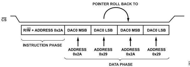
Figure 85. Looping Enabled with Address Descending and STREAM\_MODE = 2
