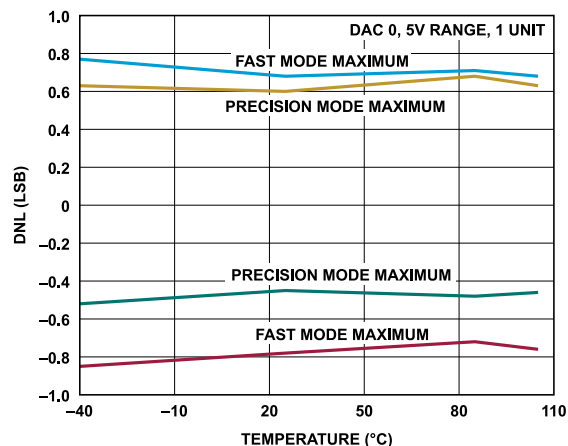
Figure 22. AD3541R-16 DNL vs. Temperature
