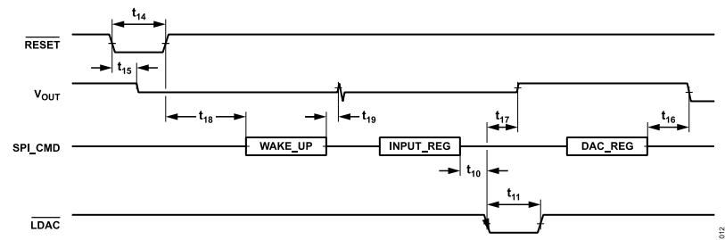
Figure 8. Start-Up Sequence Timing
