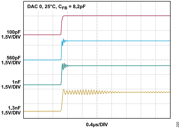
Figure 31. Output Load Stability ( C_{FB} Is Feedback Capacitor)
