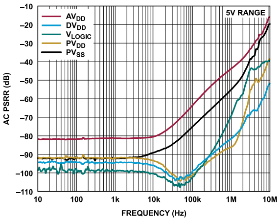
Figure 62. AC PSRR vs. Frequency
