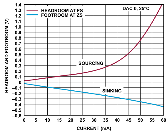
Figure 51. Headroom and Footroom vs. Load Current
