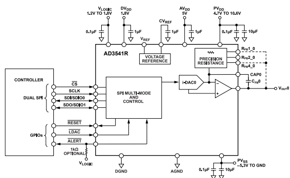
Figure 96. Recommended Application Circuit
