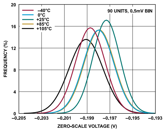
Figure 40. Zero-Scale Voltage Distribution, 0 V to 2.5 V Range
