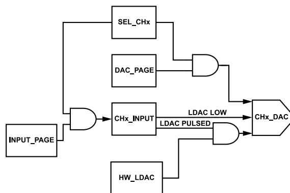
Figure 94. DAC Data Flow Between Registers
