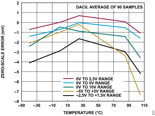
Figure 28. Zero-Scale Error vs. Temperature
