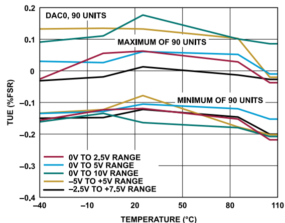
Figure 24. TUE vs. Temperature
