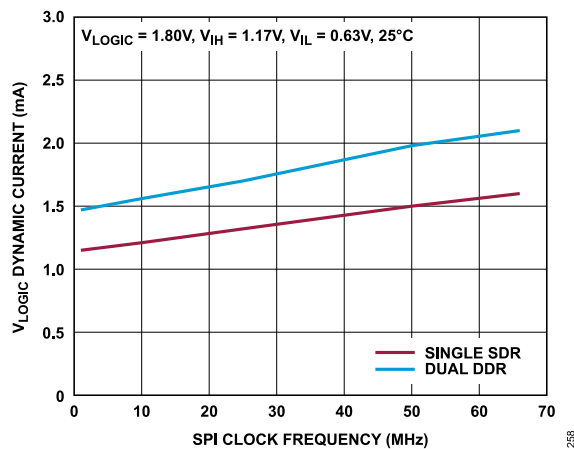
Figure 70. V_{LOGIC} Dynamic Current vs. SPI Clock Frequency, SPI Mode
