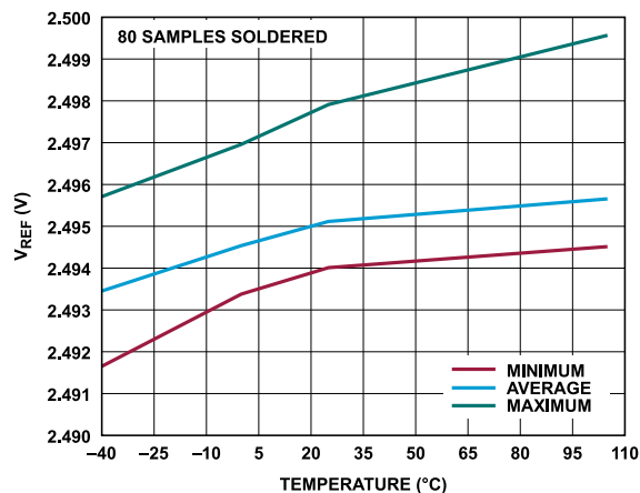
Figure 67. V_{REF} vs. Temperature
