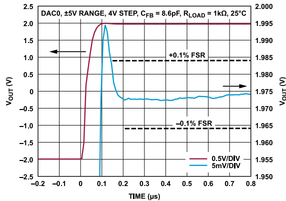
Figure 60. Large Signal Settling Time, -5 V to +5 V Range
