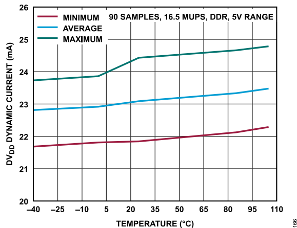
Figure 72. AD3541R-16 DV_{DD} Dynamic Current vs. Temperature
