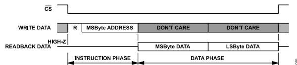
Figure 81. Multibyte Register Read with Descending Addressing
