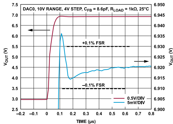
Figure 59. Large Signal Settling Time, 0 V to 10 V Range
