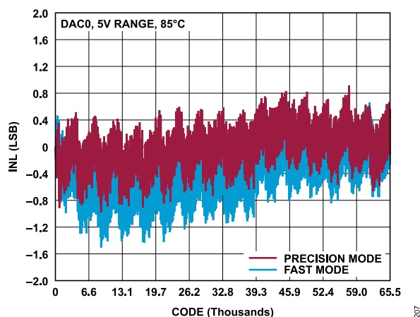
Figure 17. AD3541R-16 INL vs. Code, 0 V to 5 V Range, 85°C, Fast Mode and Precision Mode
