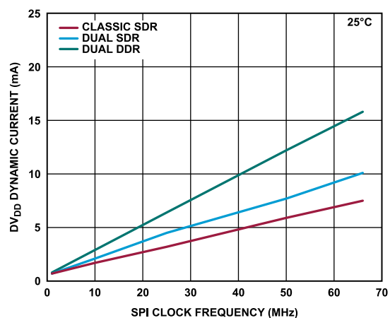
Figure 69. AD3541R-12 DV_{DD} Dynamic Current vs. SPI Clock Frequency, SPI Mode
