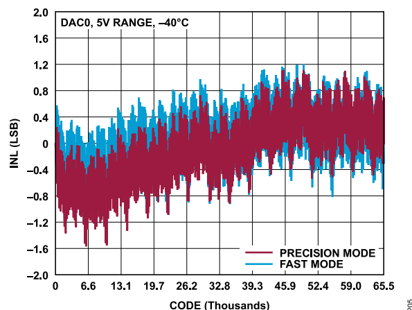
Figure 15. AD3541R-16 INL vs. Code, 0 V to 5 V Range, -40^{\circ}\text{C} , Fast Mode and Precision Mode
