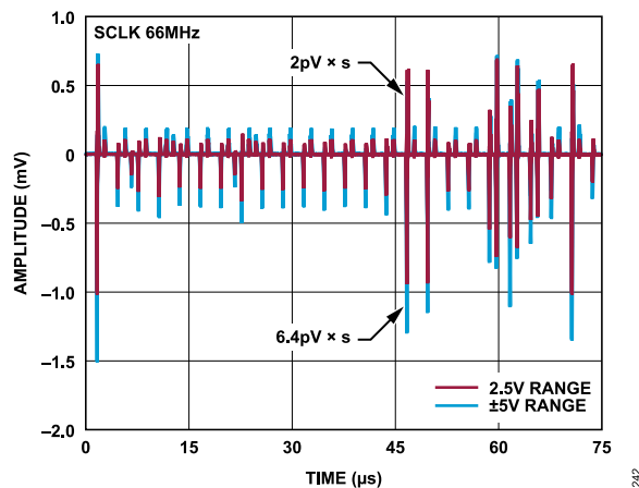
Figure 54. Digital Feedthrough
