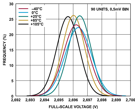
Figure 46. Full-Scale Voltage Distribution, 0 V to 2.5 V Range
