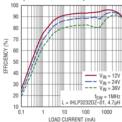
Low Load Efficiency at 5V OUT (LT8643S/LT8643SA)
