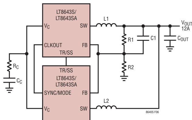
Figure 6. Paralleling Two LT8643S/LT8643SAs
