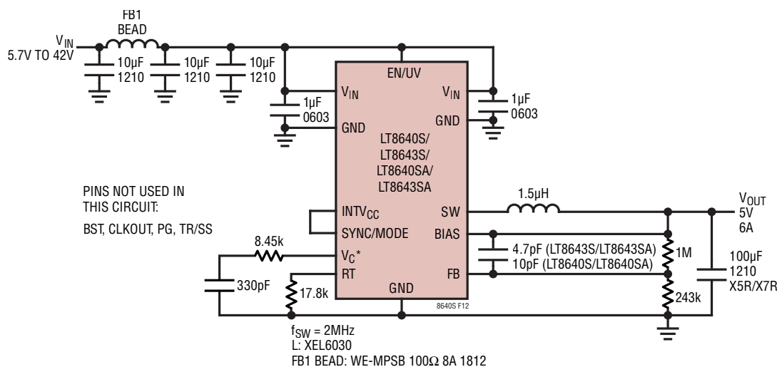
Figure 12. Ultralow EMI 5V, 6A Step-Down Converter with Spread Spectrum
