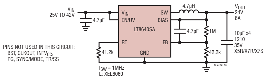
Figure 16. 24V, 6A Step-Down Converter
