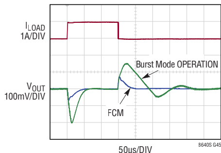
Transient Response; 100mA to 1.1A Transient (LT8640S/LT8640SA)
