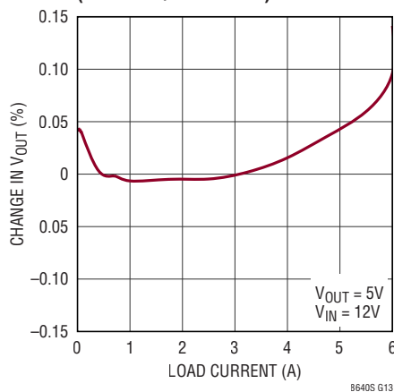
Load Regulation (LT8640S/LT8640SA)
