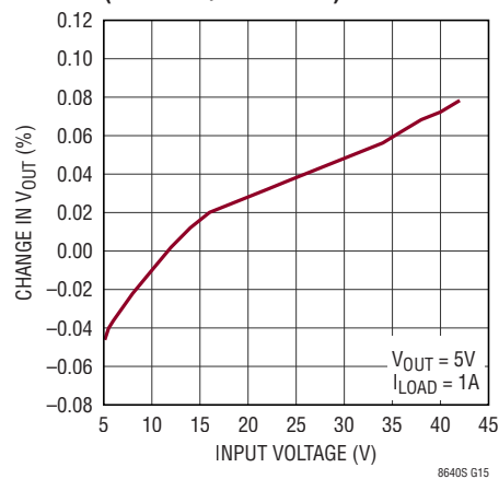
Line Regulation (LT8640S/LT8640SA)
