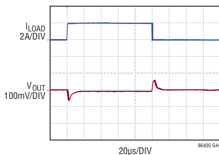
Transient Response; External Compensation (LT8643S/LT8643SA)
