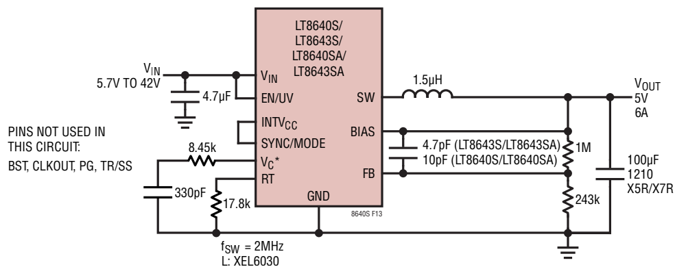
Figure 13. 2MHz 5V, 6A Step-Down Converter with Spread Spectrum
