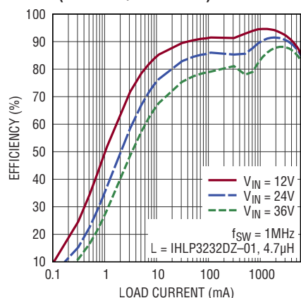
Low Load Efficiency at 3.3V OUT (LT8643S/LT8643SA)
