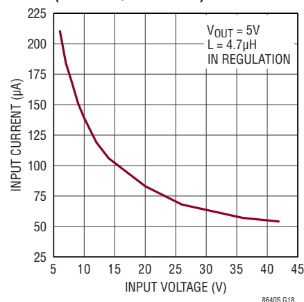
No-Load Supply Current (LT8643S/LT8643SA)
