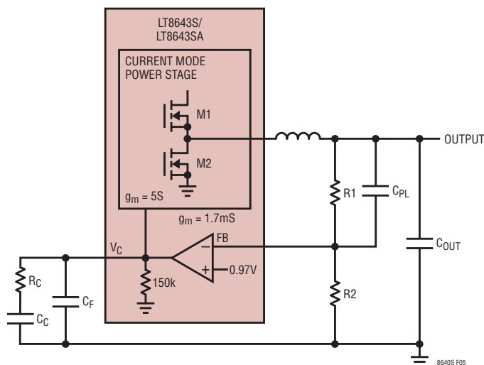
Figure 5. Model for Loop Response
