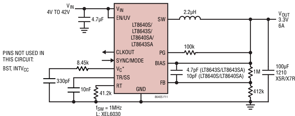
Figure 11. 3.3V, 6A Step-Down Converter with Soft-Start and Power Good
