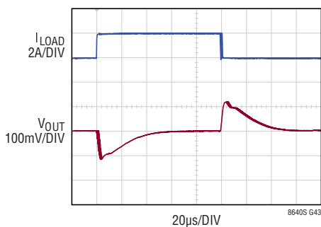
Transient Response; Internal Compensation (LT8640S/LT8640SA)
