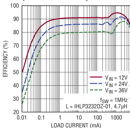
Low Load Efficiency at 3.3V OUT (LT8640S/LT8640SA)
