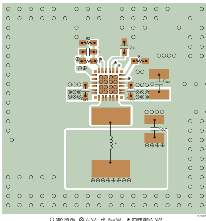
(a) LT8640S/LT8640SA
