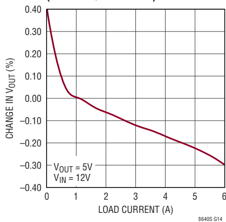
Load Regulation (LT8643S/LT8643SA)
