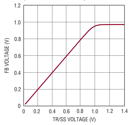
Soft-Start Tracking (LT8640S/LT8640SA)
