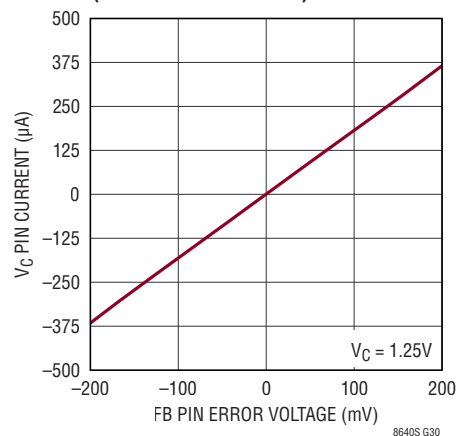
Error Amp Output Current (LT8643S/LT8643SA)
