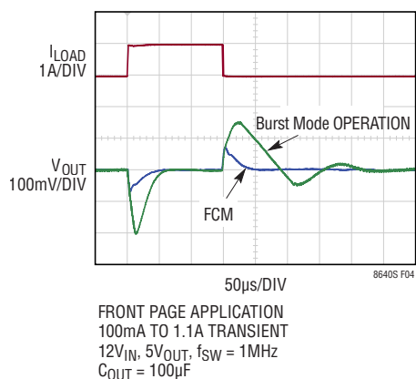
Figure 4. LT8640S/LT8640SA Load Step Transient Response with and without Forced Continuous Mode
