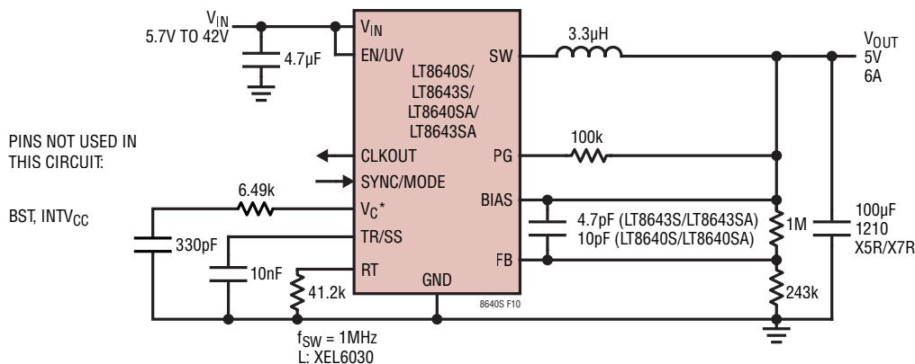
Figure 10. 5V 6A Step-Down Converter with Soft-Start and Power Good
