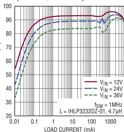
Low Load Efficiency at 5V OUT (LT8640S/LT8640SA)
