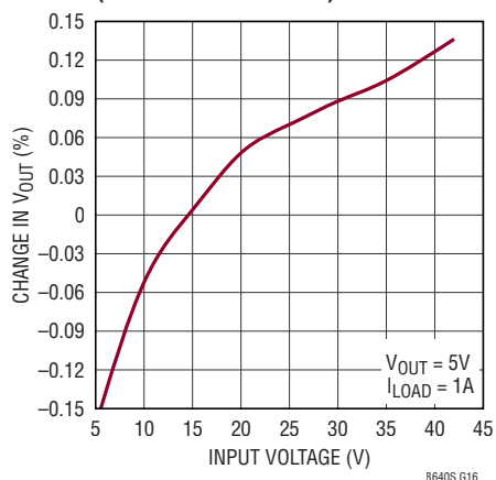
Line Regulation (LT8643S/LT8643SA)
