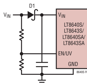
Figure 7. Reverse V_{IN} Protection
