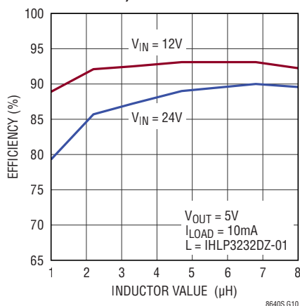
Burst Mode Operation Efficiency vs Inductor Value (LT8640S/ LT8640SA)
