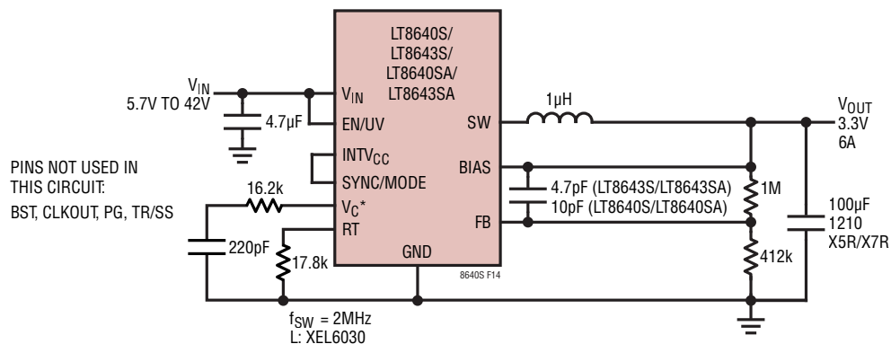
Figure 14. 2MHz 3.3V, 6A Step-Down Converter with Spread Spectrum
