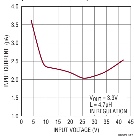
No-Load Supply Current (LT8640S/LT8640SA)
