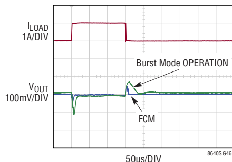
Transient Response; 100mA to 1.1A Transient (LT8643S/LT8643SA)
