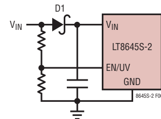
Figure 4. Reverse V_{IN} Protection
