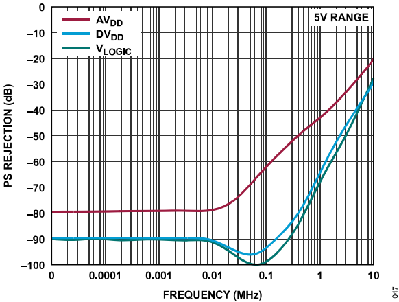
Figure 58. AC PSRR
