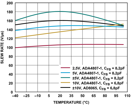
Figure 57. Slew Rate vs. Temperature
