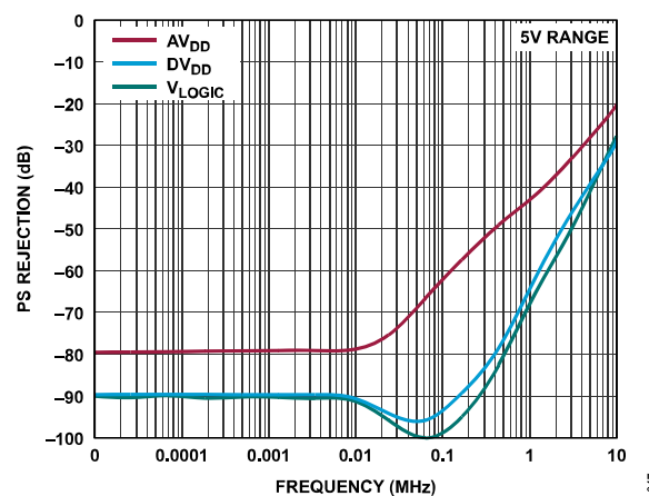
Figure 60. AC PSRR
