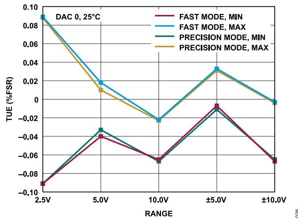
Figure 28. TUE vs. Range
