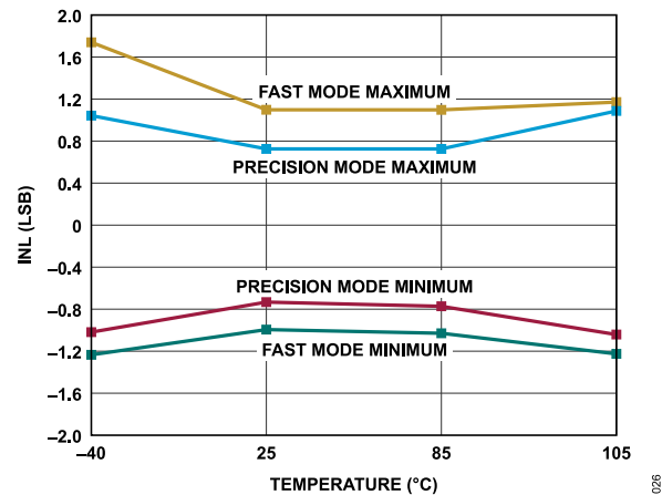
Figure 26. INL vs. Temperature
