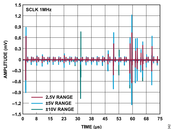
Figure 51. Digital Feedthrough
