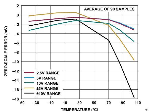
Figure 31. Zero-Scale Error vs. Temperature
